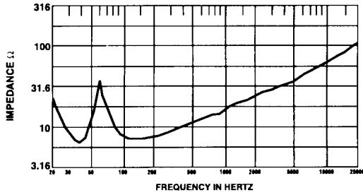
FIGURE 4 — Impedance in Typical Enclosure
