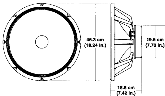
FIGURE 5 — Dimensions
