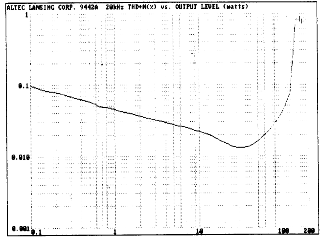
20kHz (THD + N)(%) vs LEVEL(watts)
