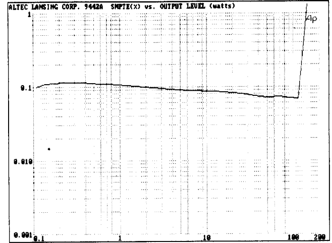
SMPTE DISTORTION(%) vs LEVEL(watts)
