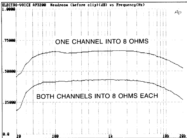
HEADROOM BEFORE CLIPPING VS. FREQUENCY
