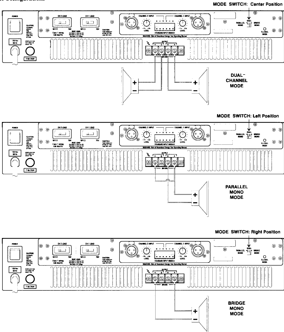
Figure 2—Output Configurations
