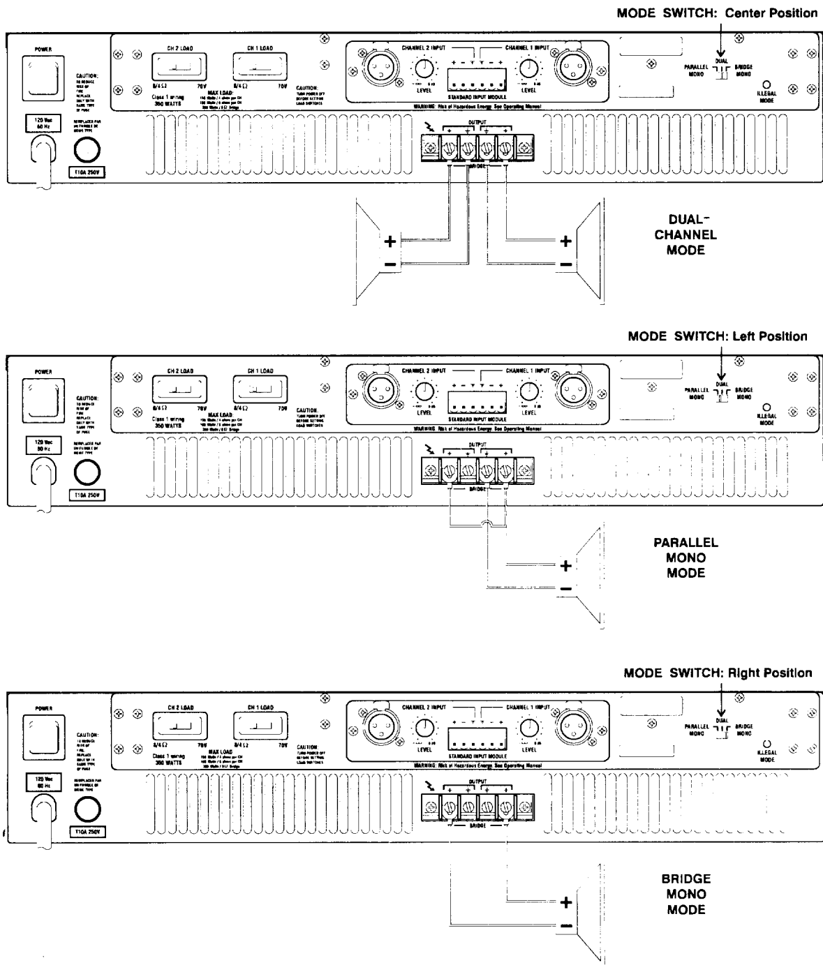
Figure 2—Output Configurations
