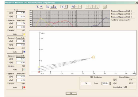
Placement window: Free speaker positioning (Y/Z axis); resulting output response shown separate or summed-up in magnitude or phase includes delays; acoustical result shown when using EV speaker files; +/-12/24/48 dB display options; display of sonic radiation at different frequencies (<150 Hz); calculated SPL; mutable output sections; different-colored outputs.
