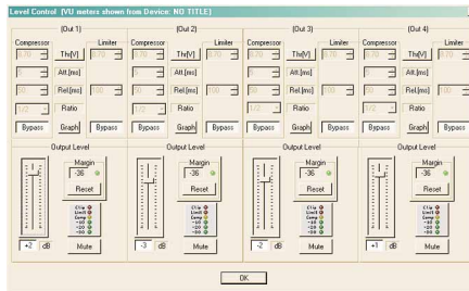
Level Control window: Level adjustment for each output; separate and bypassable compressor and limiter section with selectable threshold unit (dB/dBu/v) and graph; mute function; resettable margin indication counts amp clipping; output VU-meters display in real-time when connected to Dx38.
