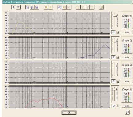
Output Frequency Response window: Level adjustment for each output; output responses shown separate in magnitude include delays and components; +/-12 dB, +/-24 dB, or +/-48 dB views; zoom function; output VU-meters display in real-time when connected to Dx38.
