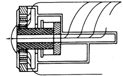
Variable-D® mic
