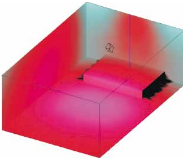
SPL radiation at 250 Hz without tripole configuration
