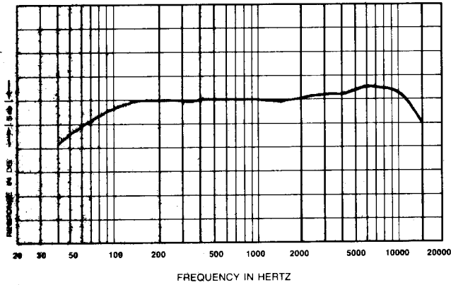
FIGURE 1 - Response Curve
