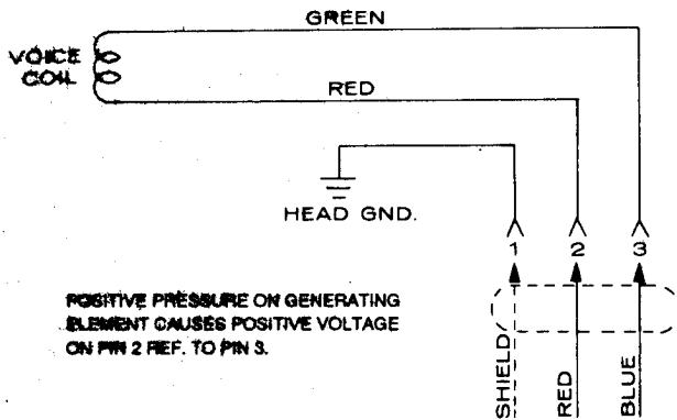
FIGURE 3 - Wiring Diagram
