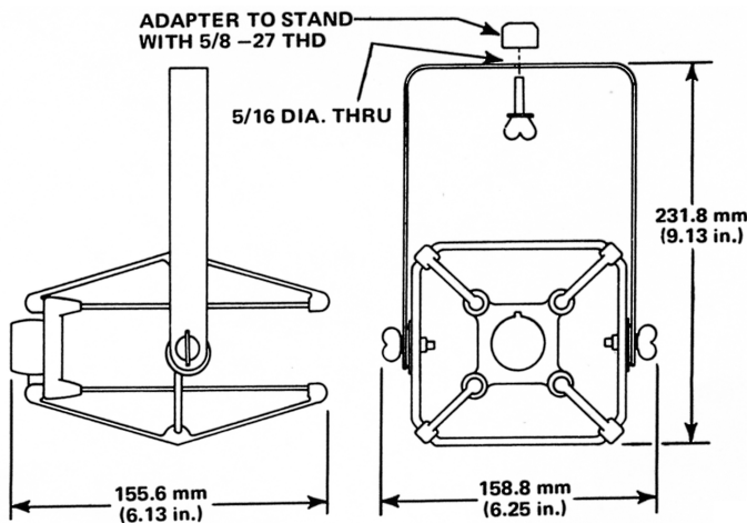
FIGURE 1—Dimensions
