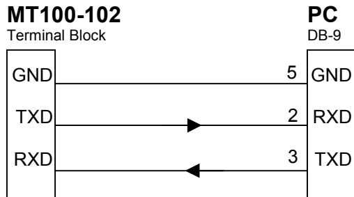
Figure 1: DB-9 Serial Connection
