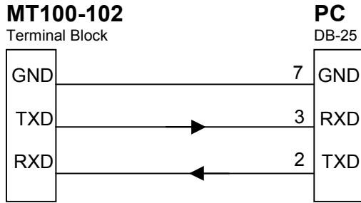
Figure 2: DB-25 Serial Connection
