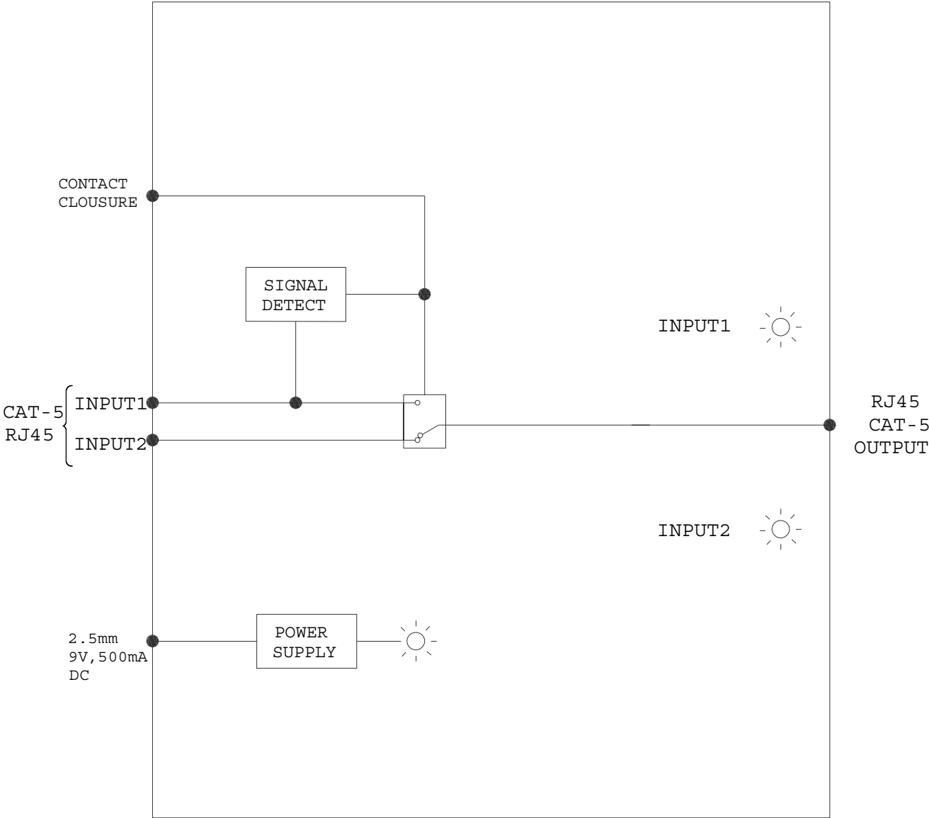
DIAGRAM 2 : INTERNAL VIEW
