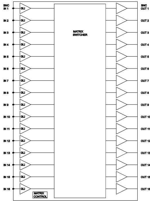
Block diagram of MT105-112/MT105-119
