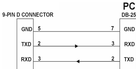
Figure 1: DB-9 Serial Connection
