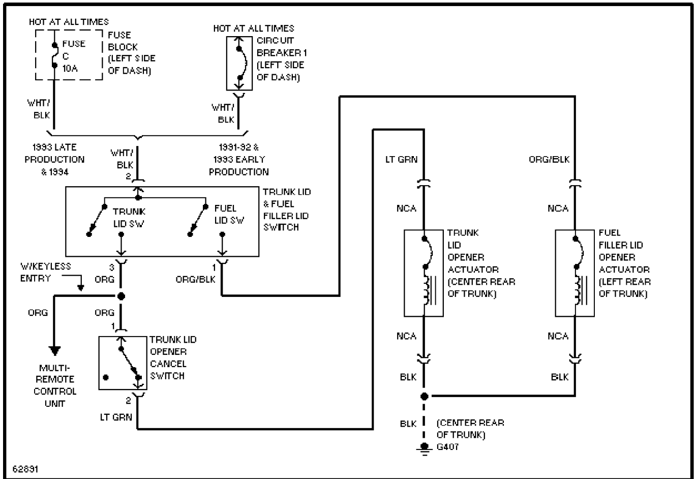
Trunk & Fuel Door Release Circuit
