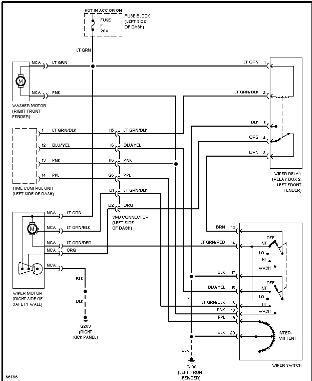
Wiper/Washer Circuit
