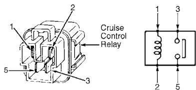
91G00790 Fig. 11: Identifying Cruise Control Relay Connector Terminals (Except 300ZX)
