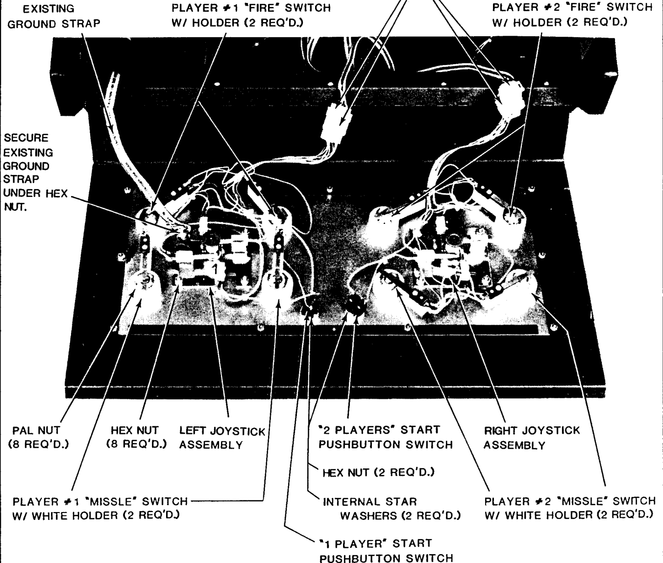
FIGURE 6. CONTROL PANEL ASSEMBLY - REAR VIEW
