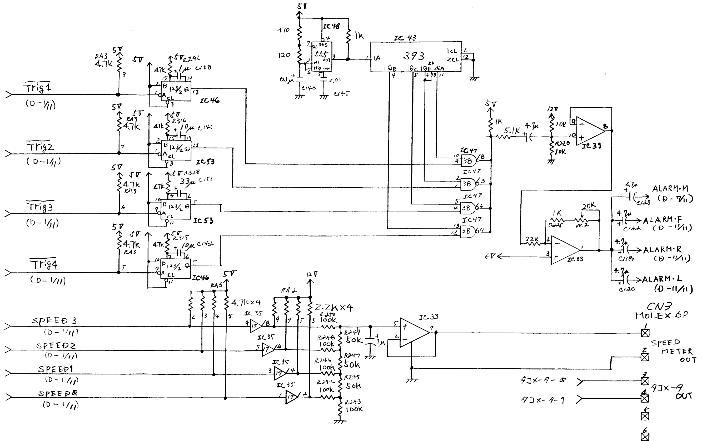
Sound Board 834-0123 Turbo Sound Alarm D-2/11 126
