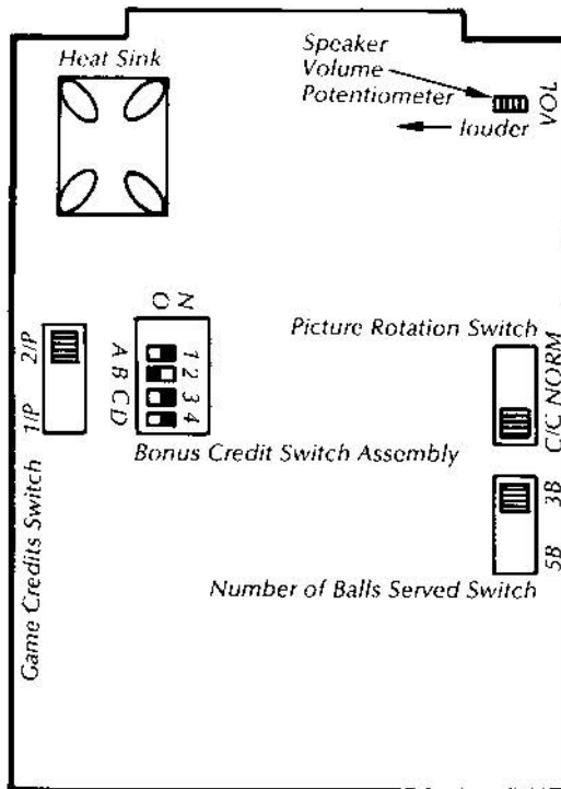
NOTE: Component side of board shown; not drawn to scale.
